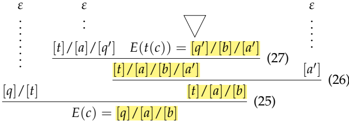
Figure 12 Fragment for a transition t = (q, a) \rightarrow (q', a') out of an existential configuration c = (q, ab) .
