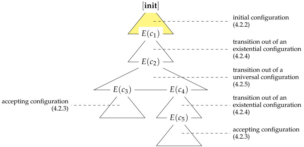
Figure 9 Schematic structure of the derivation in G that corresponds to the accepting computation in Figure 8. The derivation is displayed with the root node at the top to make the correspondence with Figure 8 more evident. Each E(c_i) is the category that encodes the configuration c_i .
