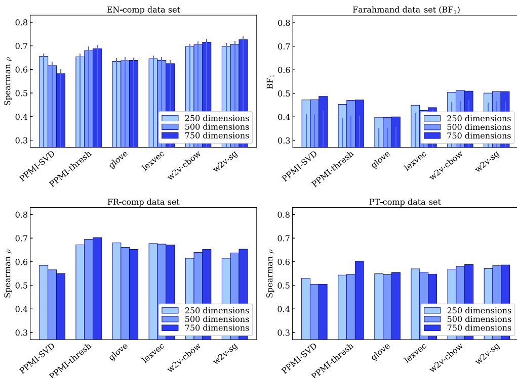
Figure 6 Best results for each DSM and DIMENSION, using BF 1 for Farahmand data set, and Spearman ρ for all the other data sets. For English, the thin bars indicate results using fallback. Differences between two highest Spearman correlations for each model are statistically significant ( p < 0.05 ), except for PPMI-SVD for FR-comp , according to Wilcoxon’s sign-rank test.
