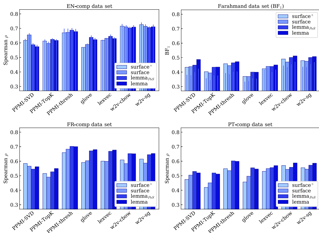
Figure 7 Best results for each DSM and WORDFORM, using BF_1 for Farahmand data set, and Spearman \rho for all the other data sets. For English, the thin bars indicate results using fallback. In EN-comp all differences between the two highest Spearman values for each DSM were significant, according to Wilcoxon’s sign-rank test, except for PPMI-thresh , while in FR-comp and PT-comp they were only significant for PPMI-TopK and lexvec .
