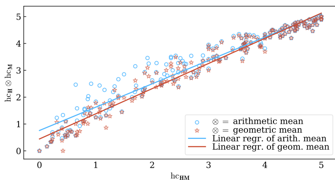
Figure 2 Relation between hc_H \otimes hc_M and hc_{HM} in FR-comp , using arithmetic and geometric means.
