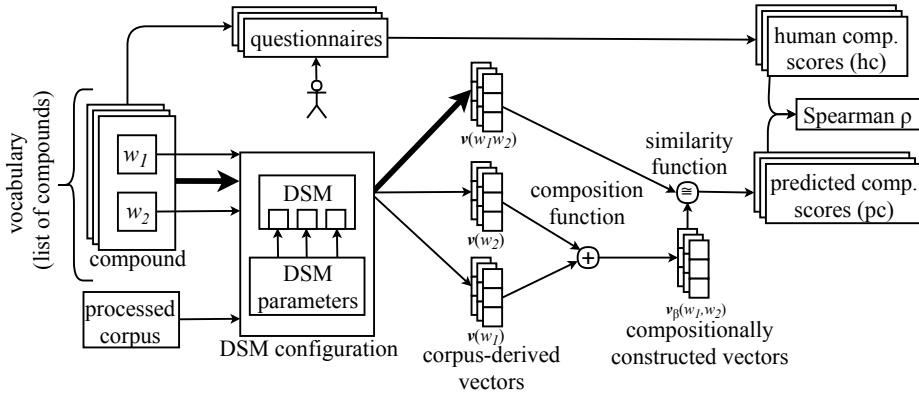
Figure 3 Schema of a compositionality prediction configuration based on a composition function. Thick arrows indicate corpus-based vectors of two-word compounds treated as a single token. The schema also covers the evaluation of the compositionality prediction configuration (top right).
