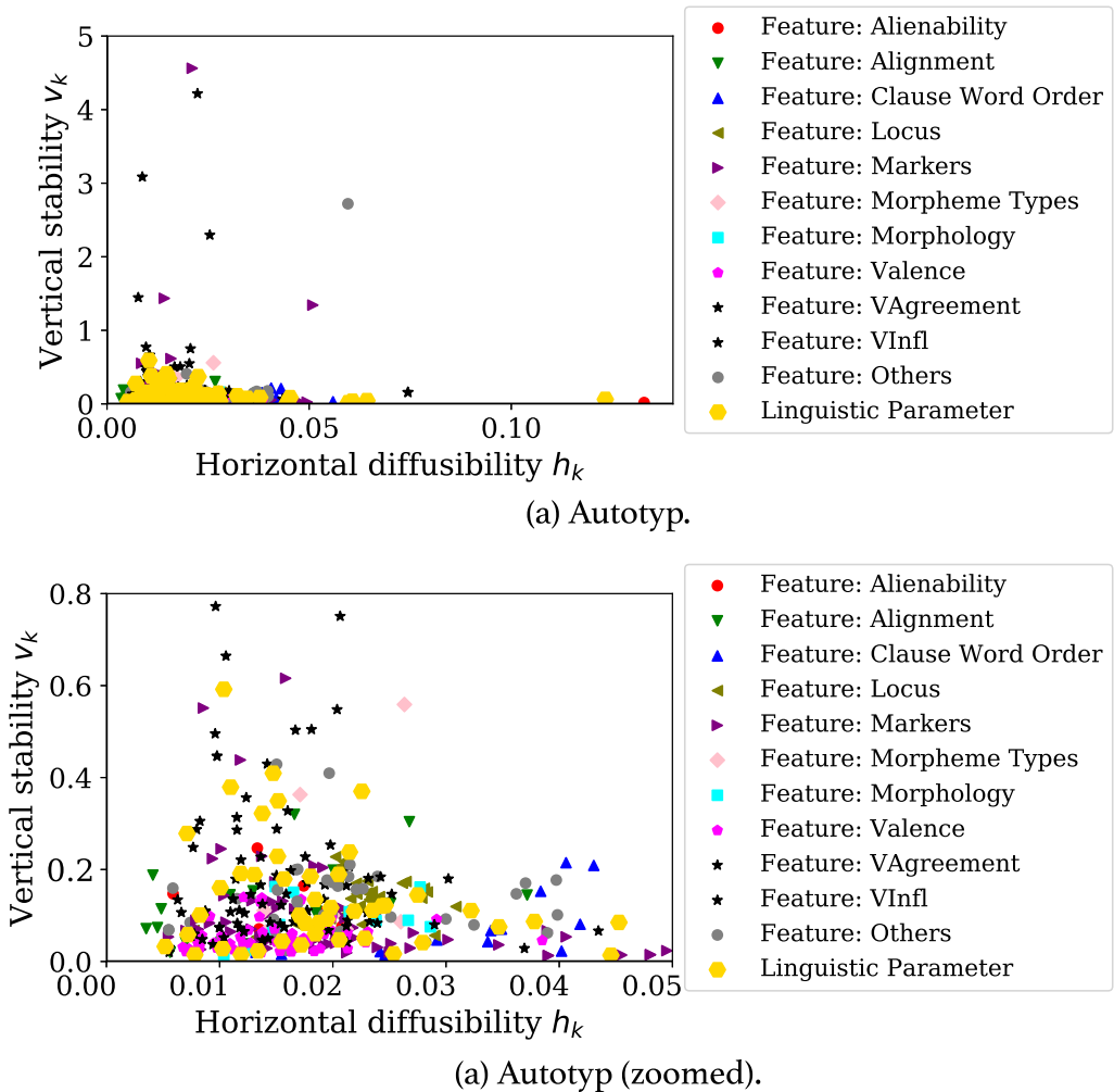
Figure 9 Scatter plots of the surface features and induced linguistic parameters of Autotyp. See Figure 8 for details.
