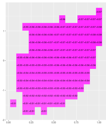
(c) ChrF3
