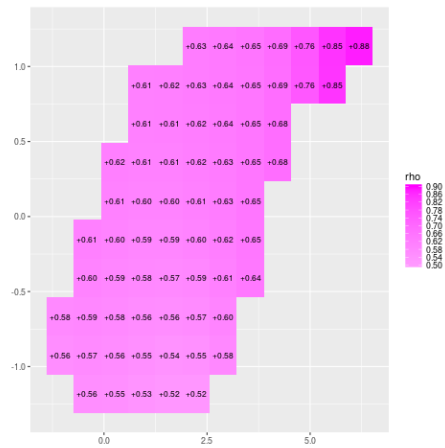
(f) Metrics-F
