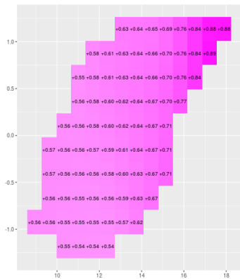
(e) DPMFcomb
