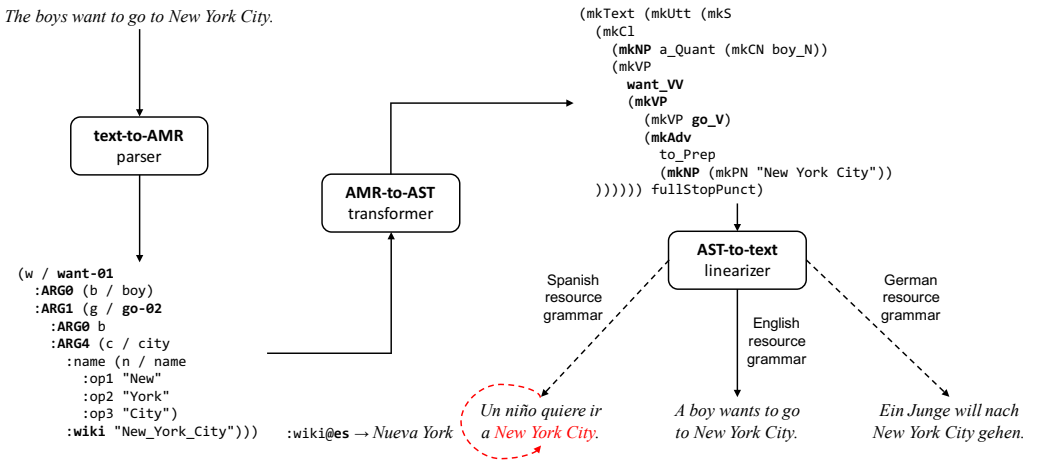
Figure 21 The overall architecture for multilingual AMR-to-text generation via GF.
