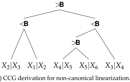
Figure 3 Relation between CCG and separating trees.
