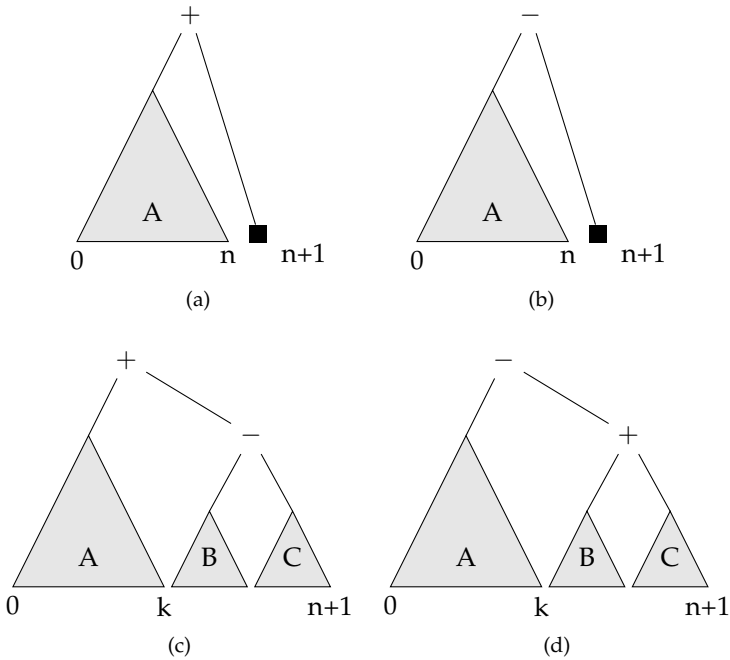
Figure 5 Normal form branching configurations.
