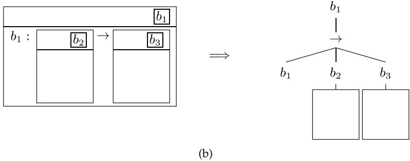
Figure 5 Example of converting a basic condition (a) and a binary complex condition (b) to a tree.
