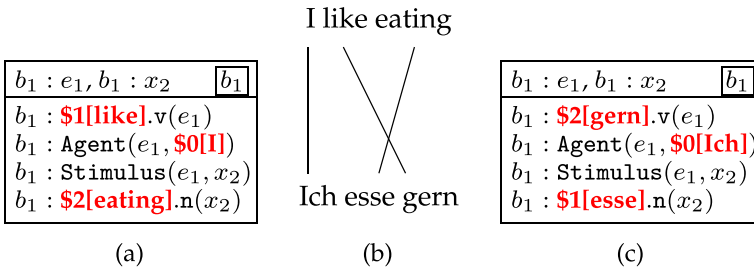
Figure 9 Example of demotional divergence. (a) UDRS of English sentence I like eating ; (b) word alignments between two sentences; (c) incorrect UDRS of German translation Ich esse gern , constructed via alignments.
