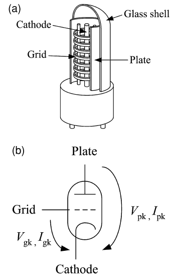
Figure 1. Physical construction (a) and electrical representation (b) of a triode tube. (Figure (a) is adapted from en.wikipedia.org/wiki/Vacuum_tube .)
