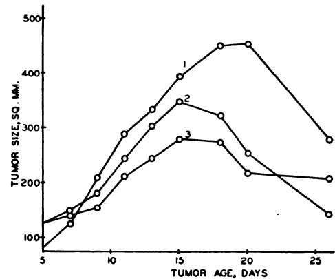
CHART 3 (Experiment V).—Curves showing the growth of Jensen sarcoma in male rats whose tumors regressed. The notations are as follows:
