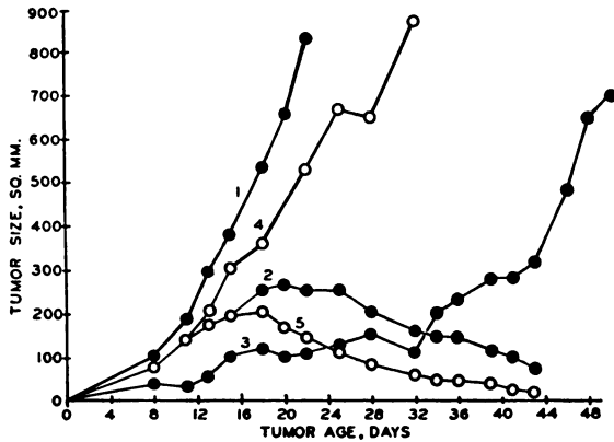
CHART 1 (Experiment I).—Curves showing the effect of ethionine on the growth of the U.C.L.A. fibrosarcoma in female rats. The notations are as follows:
