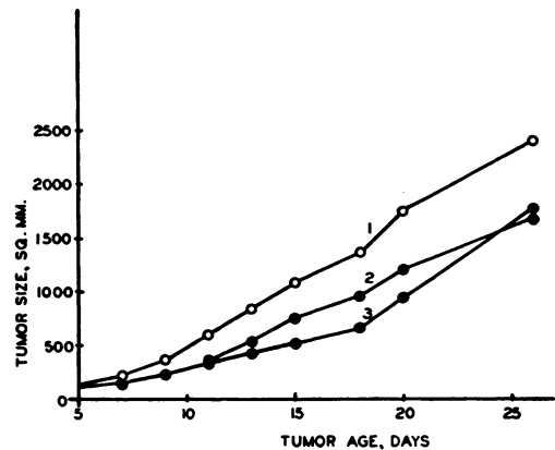
CHART 4 (Experiment V).—Curves showing the growth of Jensen sarcoma in male rats with nonregressing tumors. The notations are as follows:
