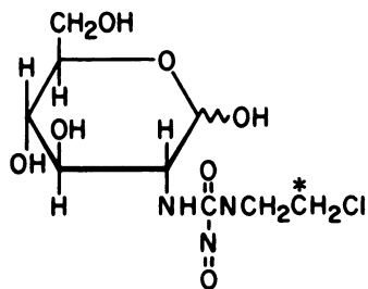
CHLOROZOTOCIN-[CHLOROETHYL-2- 14 C]
