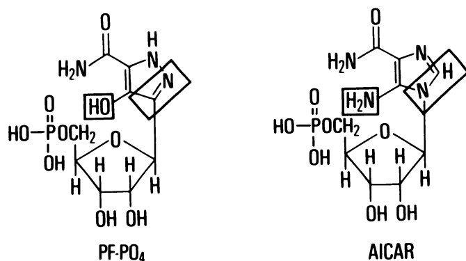
Chart 1. Structural similarity between PF-PO 4 and AICAR. The dissimilar areas of their structures are shown in the outlined areas.
