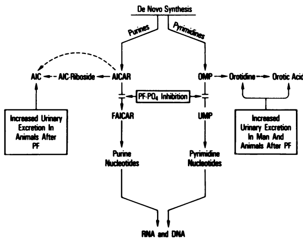
Chart 2. Inhibition of purine and pyrimidine biosynthesis by PF-PO 4 . FAICAR, formyl-AICAR; OMP, orotidine 5'-monophosphate.
