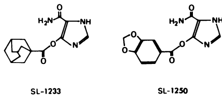
Chart 1. Chemical structures of SL-1233 and SL-1250.
