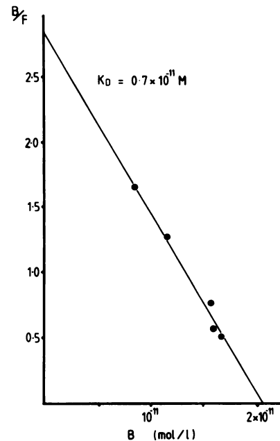
Chart 1. Scatchard analysis of binding of 1,25-(OH) 2 D 3 to cytosol from T 47D cells (see "Materials and Methods"). Receptor concentration was 150 fmol/mg cytosol protein.
