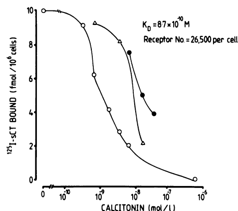
Chart 3. Binding of 125 I-labeled salmon calcitonin ( 125 I-sCT) to intact T 47D cells and competition by unlabeled salmon (O) and human (●) calcitonin, and Leu 12 -human calcitonin (Δ).
