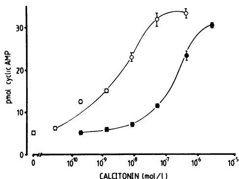
Chart 2. Effects of salmon (O) and human (●) calcitonins on adenylate cyclase activity in homogenates of T 47D cells.
