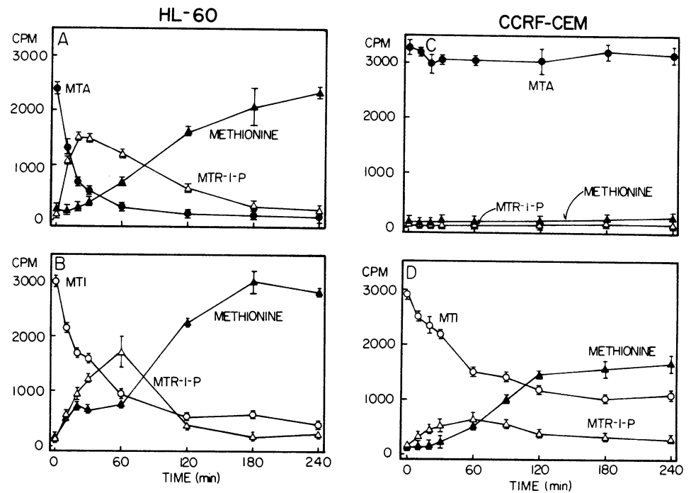
Chart 2. Conversion of [ methyl-14 C]MTA or [ methyl-14 C]MTI to MTR-1-P and methionine in sonicates of HL-60 (A and B) or CCRF-CEM (C and D). Points, mean of 2 samples run in 2 independent experiments; bars, range. Experimental details are described under "Materials and Methods."
