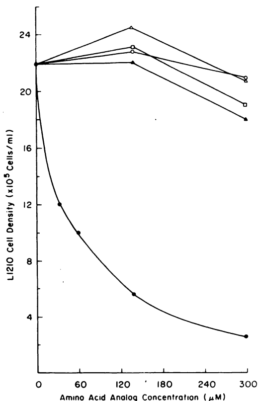
Chart 1. Actions of DL-β-amino acid analogues on L1210 cell growth. An L1210 cell suspension ( 1 \times 10^5 cells/ml) in Dulbecco's modified Eagle's medium was added to 35- x 10-mm dishes (1.5 ml/dish). After a 1-hr incubation period, each culture was treated with one of the following amino acid analogues: ●, DL-threo-β-F-Asn; ▲, DL-erythro-β-F-Asn; □, DL-threo-β-OH-Asn; ○, DL-threo-β-F-Asp·HCl; and △, DL-erythro-β-F-Asp·HCl; and incubation was continued for 45 hr. After this period, the cell number was counted. The values shown represent means of duplicate dishes with a maximum range equal to ±15%.
