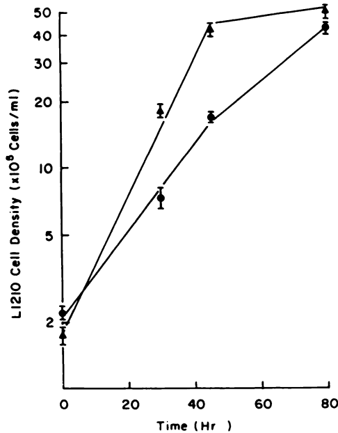
Chart 4. Growth of L1210 cells following DL-threo-β-F-Asn removal. An L1210 cell suspension (1.5 × 10 6 cells/ml) in Dulbecco's modified Eagle's medium was divided equally; one half was treated with DL-threo-β-F-Asn at a final concentration of 300 μM. The other half served as an untreated control. These cell suspensions were seeded into 35- × 10-mm dishes (2.2 × 10 6 cells/dish) and incubated for 40 hr. The cell numbers after this period were 1.5 × 10 6 cells/ml for the controls and 2.9 × 10 6 cells/ml for the treated group. The cell suspensions from 5 control dishes and 15 treated dishes were pooled separately into sterile centrifuge tubes and diluted to 20 ml with sterile Dulbecco's modified Eagle's medium, and the cells were pelleted by centrifugation. The supernatant medium was removed, and the cells were resuspended in Dulbecco's modified Eagle's medium to a density of 2 × 10 6 cells/ml. These cell suspensions were divided into 35- × 10-mm dishes (3 × 10 6 cells/dish) and incubated for 80 hr. At the time intervals indicated, 2 dishes from each group were used to determine cell number. ▲, untreated; ●, treated. Bars, S.D.
