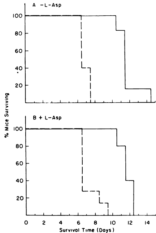
Chart 5. Survival curves for untreated and treated mice bearing L1210 cells. Twenty-four hr after tumor cell injection, treatment with DL-threo-β-F-Asn was initiated with 2 injections (0.4 ml, i.p.) per day (10 a.m., 3 p.m.), each containing 250 mg/kg. Treatment was continued for 12 days. Neutralized saline for untreated controls and neutralized DL-threo-β-F-Asn solutions were used in this experiment (see "Materials and Methods"). A, treatment with DL-threo-β-F-Asn only. The untreated control and treated groups each contained 6 animals. B, treatment with DL-threo-β-F-Asn + L-Asp (1500 mg/kg). The untreated control group contained 7 animals; the treated group contained 5 animals. In A, the mean survival times were: 7.4 ± 0.5 days (S.D.) for the untreated control group and 12.3 ± 1.4 days for the treated group. In B, the mean survival times were: 7.7 ± 1.3 days for the untreated control group and 12.2 ± 1.0 for the treated group. —, treated group; ---, untreated group.
