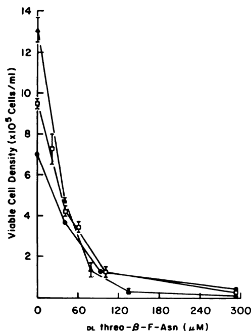
Chart 2. Growth inhibition of human leukemia cells by DL-threo-β-F-Asn. RPMI 8226, CCRF-SB, and IM-9 cells were seeded in 35- x 10-mm dishes containing 1.5 ml of RPMI 1640 medium depleted in L-Asp and L-Asn for RPMI 8226 and IM-9 cells and minimal essential medium for CCRF-SB cells at an initial density of 2.4 \times 10^5 cells/ml (>95% viability). Two hr after seeding, the cells were treated with various concentrations of DL-threo-β-F-Asn. After 3.5 days, the cells were counted, and the viability was determined. ▲ IM-9; ●, CCRF-SB; □, RPMI 8226. Bars, S.D.
