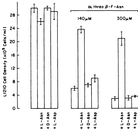
Chart 3. Prevention of DL-threo-β-F-Asn growth inhibition by L-Asn. An L1210 cell suspension (1 × 10 5 cells/ml) in Dulbecco's modified Eagle's medium was added to 35- × 10-mm dishes (1.5 ml/dish). After 1-hr incubation period, the dishes were divided into 3 groups, and each group was treated without or with DL-threo-β-F-Asn at 140 or 300 μM final concentrations. Within each group, cultures were treated with 1 mM L-Asn, D-Asn, or L-Asp. After a 48-hr incubation period, the cell number was counted. Bars, mean of duplicate dishes; brackets, range.
