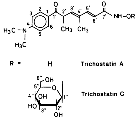
Fig. 1. Structures of trichostatin A and C.
