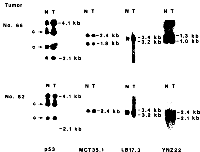
Fig. 6. Southern blot analysis for the tumors demonstrating potential existence of two regions of chromosome 17p. Tumor 66 showed only LOH (1.3-kilobase band) of YNZ22, but both alleles were retained with p53, MCT35.1, and LB17.3. Tumor 82 showed only LOH (4.1-kilobase band) of the p53 gene, but both alleles were retained with YNZ22 and LB17.3. MCT35.1 was not informative in this tumor. Arrows (C), the constant band.
