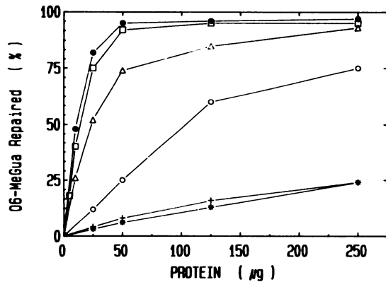
Fig. 1. Removal of O 6 -methylguanine ( O 6 -MeGua) from alkylated DNA by H4 cell extracts. [ 3 H]MNNU-treated DNA was incubated with extracts from control (O), γ-irradiated (3 Gy) (●), cis -DDP-treated (5 μM, 1 h) (Δ), or 2-methyl-9-hydroxyellipticinium-treated (2.5 μM, 1 h) (□) cells. The transferase activity was measured in cells grown for 48 h in normal medium after these treatments. Additionally, control (+) or preirradiated cells (3 Gy) (*) were incubated for 3 h with O 6 -methylguanine (1 mM) before transferase activity determination.
