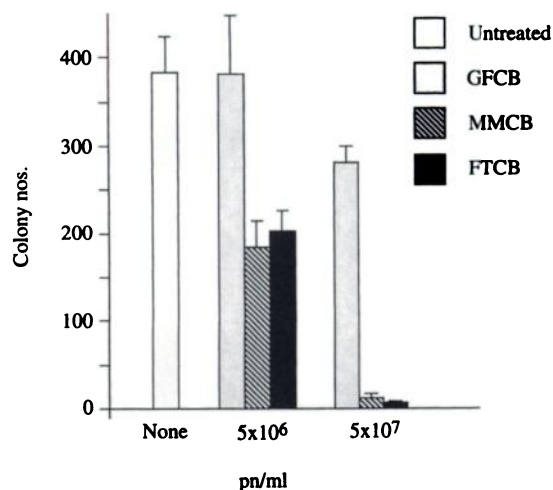
Fig. 4. Soft-agar colony formation. U87MG cells were infected with MMCB, GFCB, or FTCB at the indicated concentrations for 24 h. Mean colony numbers are plotted; bars, SD (three replicates).
