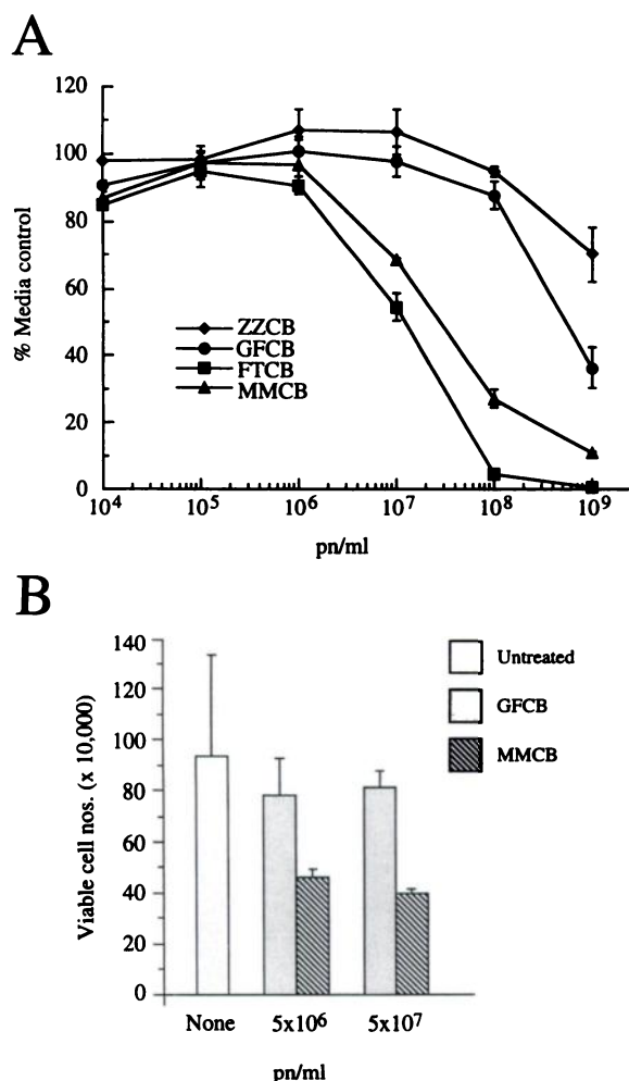
Fig. 3. Inhibition of in vitro proliferation by MMCB. A , [ 3 H]thymidine uptake. U87MG cells were infected with MMCB or control Ads at the indicated concentrations for 24 h. Results are plotted as percentages of medium-treated control (mean \pm SD). B , viable cell count assay. U87MG cells were infected with MMCB or GFCB as in A . Mean cell numbers at 72 h after infection are plotted; bars, SD (three replicates).
