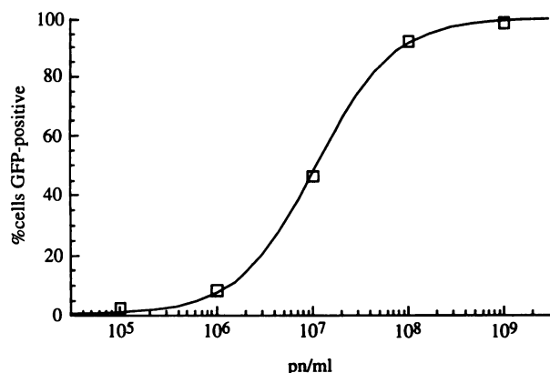
Fig. 2. FACS infectivity assay. U87MG cells were infected with GFCB at the indicated concentrations for 24 h. The fraction of cells expressing green fluorescent protein was quantitated by flow cytometry.
