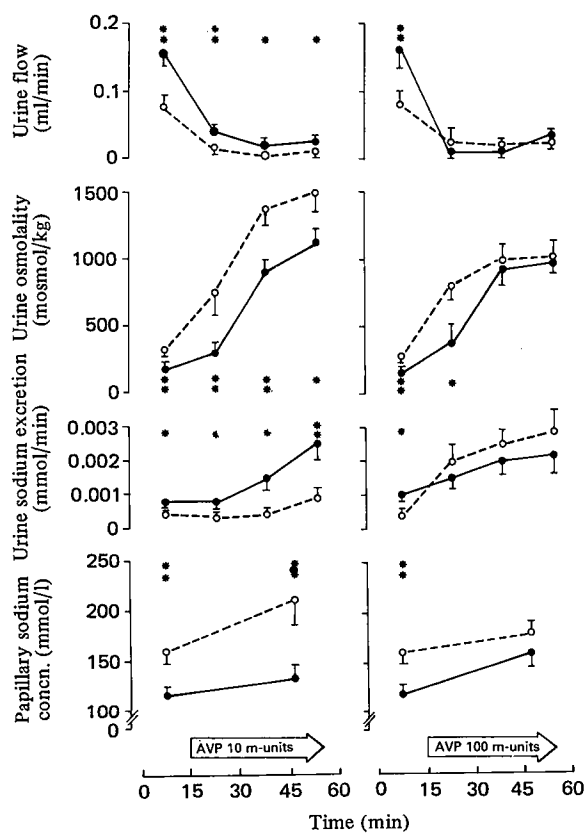
FIG. 1. Effect of vasopressin (AVP: 10 and 100 m-units) on urine flow, osmolality and sodium excretion and also papillary sodium concentration in control (●—●) and indomethacin treated (○- - -○) rats. Significantly different between control and indomethacin groups: * P < 0.05 ; ** P < 0.01 .
