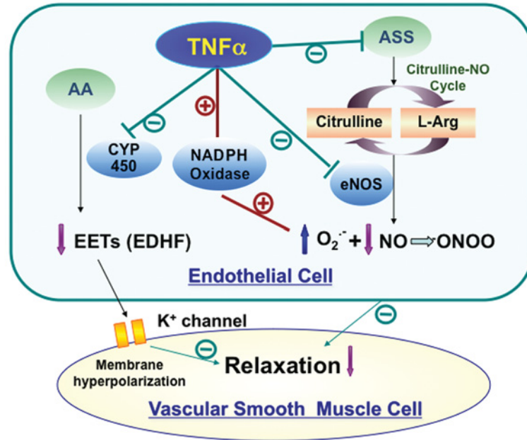
Figure 2 Role of TNF- \alpha in endothelial dysfunction
