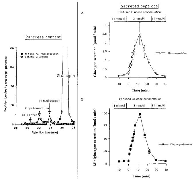
FIG. 3. Left panel: analysis by HPLC/radioimmunoassay of an extract of rat pancreas using the heat coagulation/acid extraction method followed by separation of the peptides by HPLC and analysis by glucagon and miniglucagon radioimmunoassays. Data are from reference 6. Right panel: effect of a decrease in extracellular glucose concentration on glucagon (A) and miniglucagon (B) secretion from the perfused rat pancreas. The results are expressed as amounts of glucagon and miniglucagon secreted per minute and represent the mean \pm SE of four independent experiments. Measuring the AUCs for glucagon and miniglucagon indicates that, on a molar basis, the latter is secreted at 3.48% of the former, as a mean.
