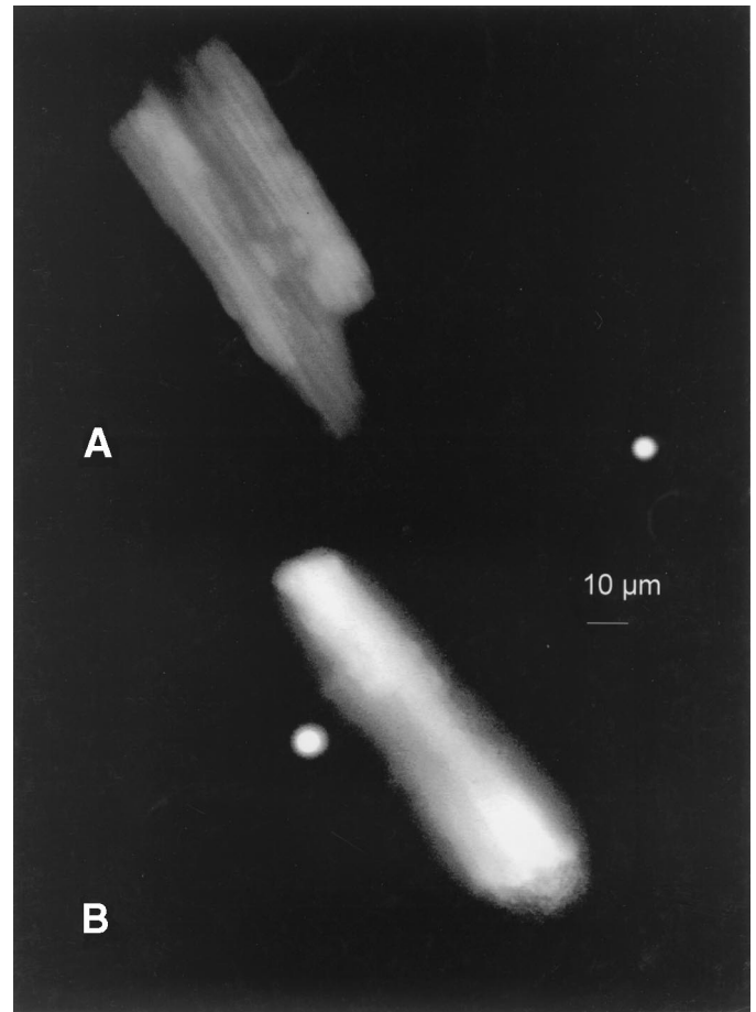
FIG. 4. Representative cardiomyocytes after incubation with CM- H_2DCFDA for 30 min. A: Myocyte in M199 medium. B: Myocyte in M199 medium treated with H_2O_2 (40 \mu\text{mol/l} ).
