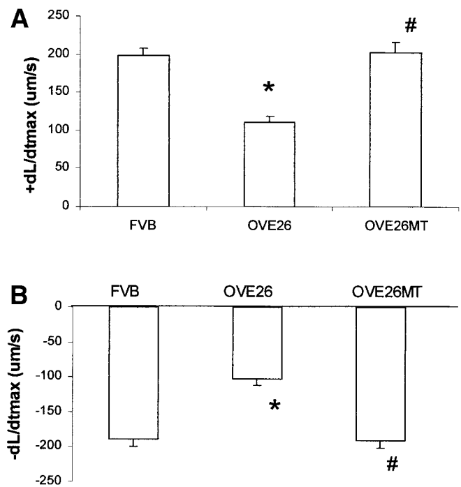
FIG. 2. Slow contraction and relaxation rates in OVE26 but not in OVE26MT cardiomyocytes. Maximal velocities of cell shortening ( +dL/dt ; A) and relengthening ( -dL/dt ; B) in ventricular myocytes isolated from FVB, OVE26 diabetic, and OVE26MT mouse hearts. Mean \pm SE, n = 60 cells/group, six mice/group. * P < 0.01 vs. FVB group; # P < 0.01 vs. OVE26 group.
