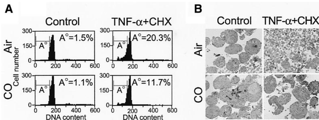
FIG. 3. Exogenous CO protects murine islets of Langerhans from apoptosis. A: Apoptosis was induced in freshly isolated murine islets (C57BL/6) by stimulation with TNF- \alpha and CHX. Immediately after stimulation, islets were exposed to exogenous CO (15) for 24 h. Control islets were treated in the same manner but not exposed to CO. After 48 h, cells were analyzed on a FACScan for DNA fragmentation. This experiment was done twice with indistinguishable results. B: Islets were treated as described in Fig. 3A and then fixed, embedded in plastic, and stained with toluidine blue for histopathologic evaluation.
