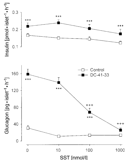
FIG. 2. The effect of 2 \mu mol/l DC-41-33 on the insulin and glucagon responses to 20 mmol/l arginine in the presence of increasing concentrations of SST, in batch incubations of isolated islets. Results are expressed as mean \pm SE of three experiments (three to five observations per experiment). *** P < 0.001 vs. without DC-41-33; **** P < 0.001 vs. 0 nmol/l SST + 2 \mu mol/l DC-41-33.
