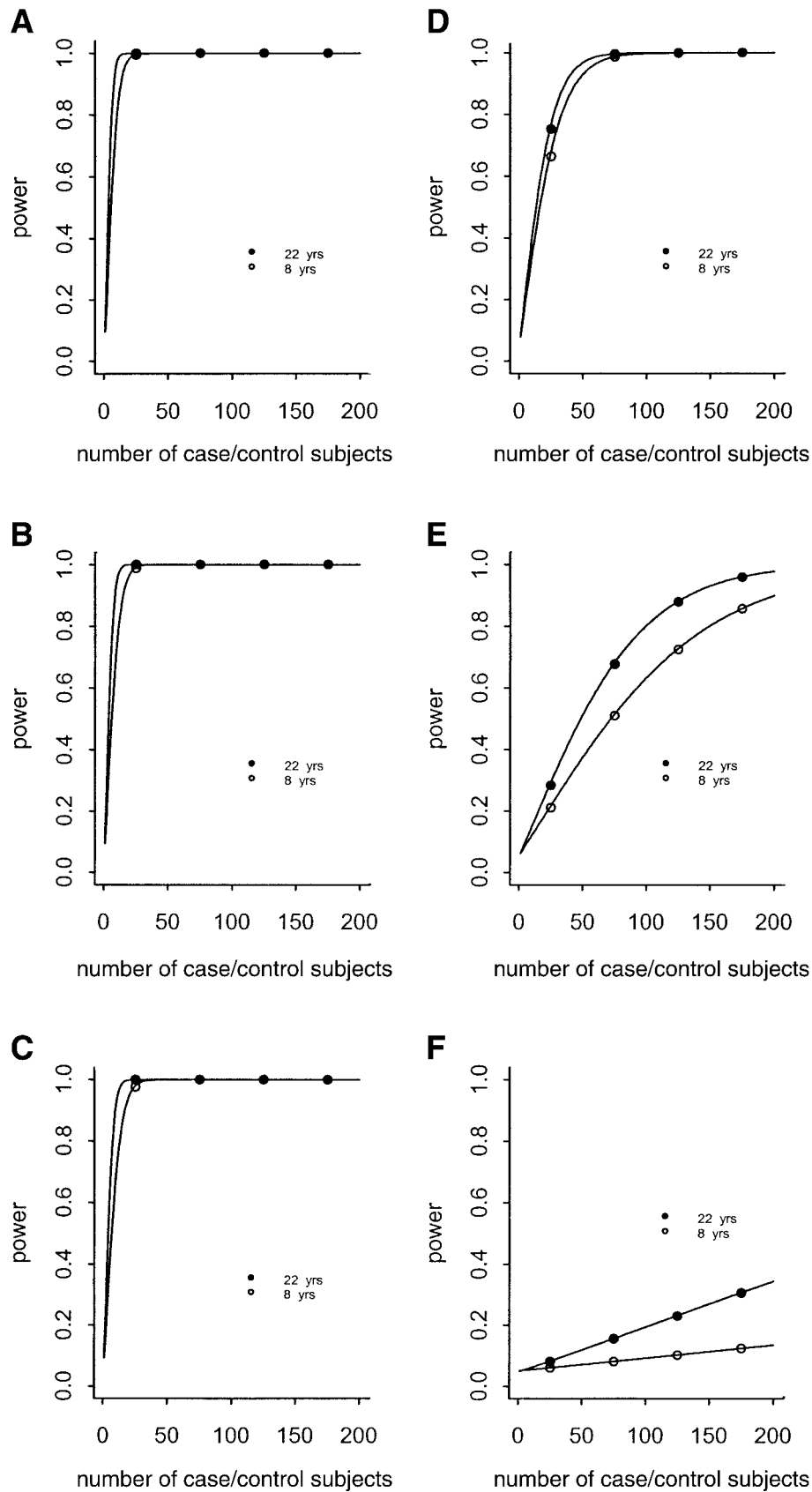
FIG. 3. Power of case-control analysis to detect major (A) or minor (D) gene when case subjects developed proteinuria after 10 years of diabetes and control subjects without proteinuria had diabetes duration of 8 or 22 years. Power of case-control analysis to detect major (B) or minor (E) gene when case subjects developed proteinuria after 15 years of duration of diabetes and when control subjects without proteinuria had diabetes duration of 8 or 22 years. Power of case-control analysis to detect major (C) or minor (F) gene when case subjects developed proteinuria after 17 years of duration of diabetes and when control subjects without proteinuria had diabetes duration of 8 or 22 years.
