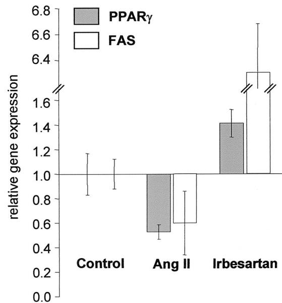
FIG. 3. Expression analysis of the adipogenic marker genes encoding PPAR \gamma and FAS in preadipocytes at day 8 after induction of differentiation with insulin + hydrocortisone + T_3 . Expression levels of cells differentiated in the presence of 10 \mu\text{mol/l} Ang II ( AT_1 receptor agonist) or 10 \mu\text{mol/l} irbesartan ( AT_1 receptor antagonist) were compared with those differentiated without irbesartan or Ang II (control). Data are means of quadruplicate determinations during a single experiment.
