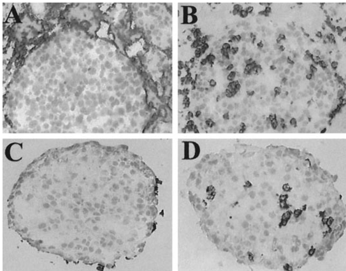
FIG. 4. Human islets incubated in tubing loops filled with ABO-compatible blood containing Melagatran at 0.4 \mu\text{mol/l} (A and B) or 10 \mu\text{mol/l} (C and D). The figure shows the distribution of platelets and leukocytes after staining with monoclonal anti-CD41a (A and C) and anti-CD11b + (B and D), respectively.
