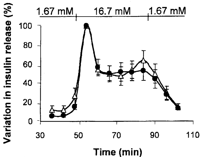
FIG. 1. Islet function tested in a dynamic perfusion system. Islets from three different pancreata were cultured in the presence ( \Delta ) and absence ( \bullet ) of 10 \mu\text{mol/l} Melagatran for 3 days. The figure shows insulin release from the islets after stimulation with glucose (1.67, 16.7, and 1.67 mmol/l).
