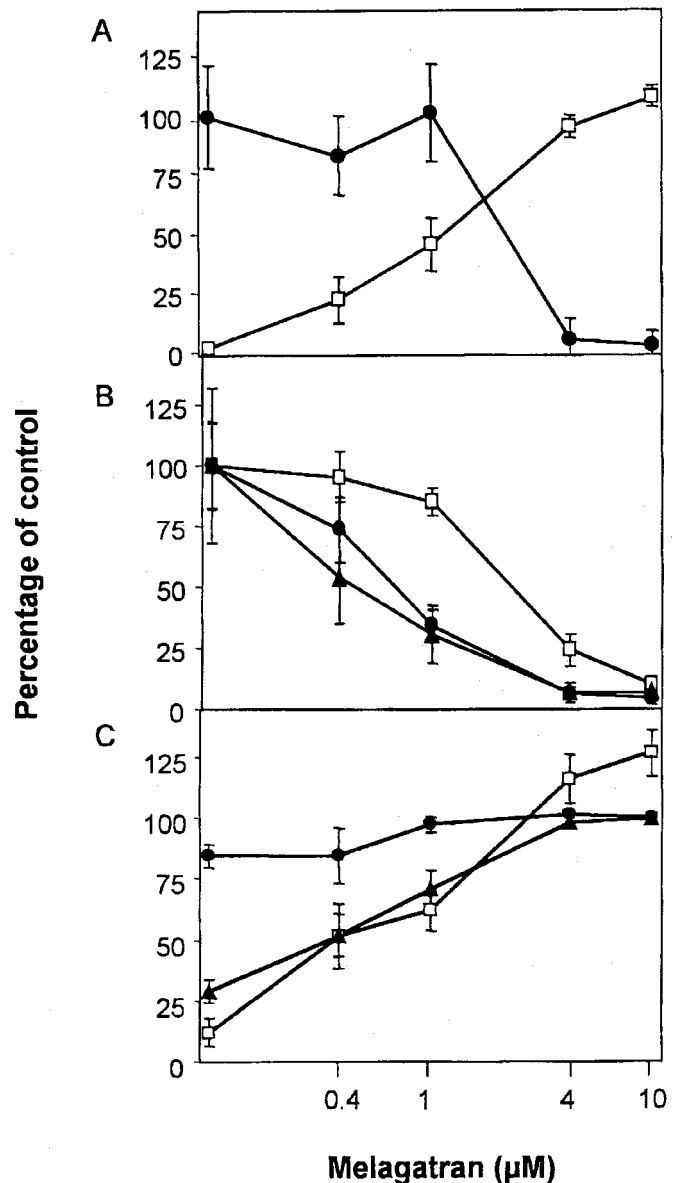
FIG. 2. Human islets incubated in the tubing loop model filled with ABO-compatible blood containing Melagatran at concentrations ranging from 0 to 10 \mu\text{mol/l} . A: Changes in platelet particle count ( \square ) and the release of \beta -TG ( \bullet ). B: Changes in prothrombin fragments 1 and 2 ( \square ), TAT ( \bullet ), and FXIa-AT ( \blacktriangle ). C: Changes in lymphocyte ( \bullet ), monocyte ( \square ), and PMN ( \blacktriangle ) particle counts. The EIA values represent data minus the medium control (no islets or Melagatran) after 60 min and are expressed as percentage of the values for the untreated control containing human islets but no Melagatran. The cell counts are expressed as percentage of the values for the medium control (no islets or Melagatran).
