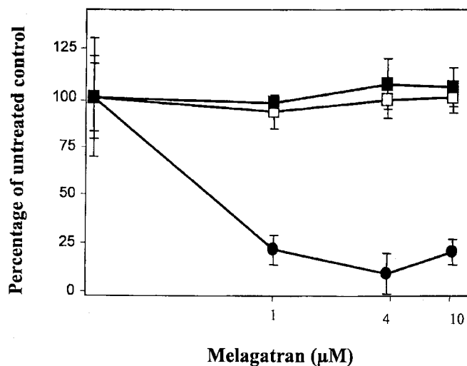
FIG. 3. Effect of Melagatran on the complement system. Changes in the generation of soluble C3a (□) and bound C3 fragments (■) in a serum model with no islets present, and changes in soluble C3a (●) in the tubing loop model containing islets in ABO-compatible blood with Melagatran at concentrations of 0–10 \mu\text{mol/l} .
