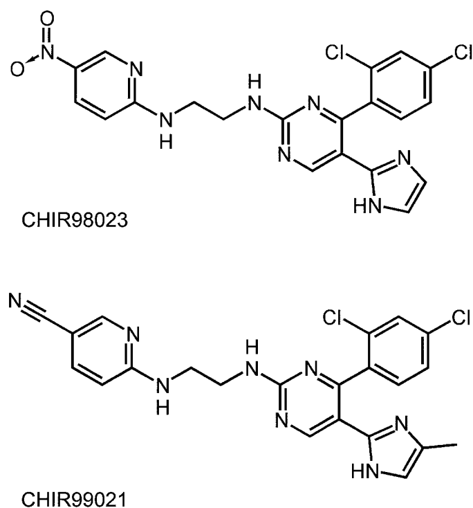
FIG. 1. Molecular structures of the GSK-3 \beta inhibitors CHIR98023 and CHIR99021.
