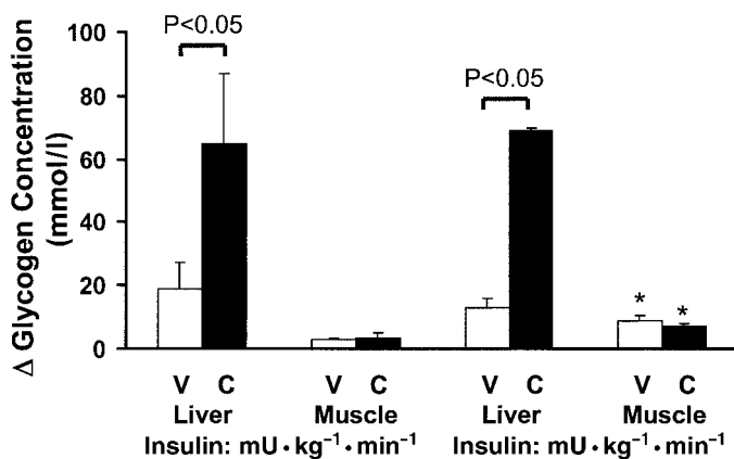
FIG. 5. Change in glycogen concentration in liver and gastrocnemius muscle in ZDF ( fa/fa ) rats treated with vehicle (□) or CHIR99021 (■) after euglycemic-hyperglycemic clamps at insulin infusion rates of 2 or 20 mU · kg -1 · min -1 . * P < 0.05 compared with muscle glycogen concentrations after the 2-mU · kg -1 · min -1 clamp.
