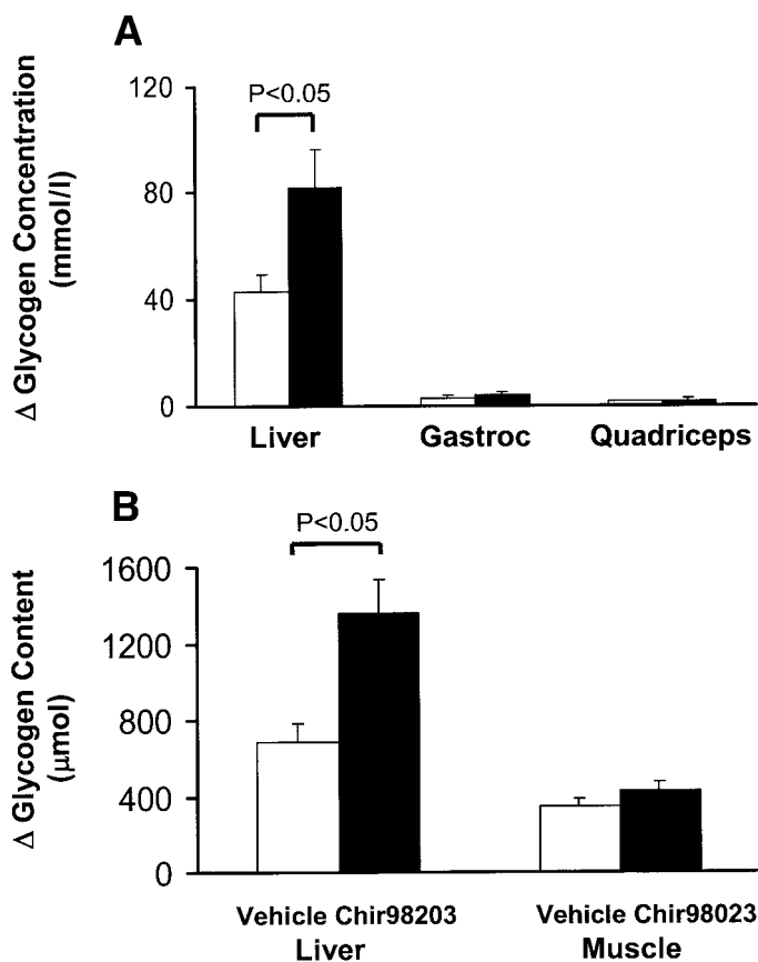
FIG. 4. A: Change in glycogen concentration in liver, gastrocnemius, and quadriceps muscle in ZDF ( alfa ) rats treated with vehicle (□) or CHIR98023 (■) after an OGTT. B: Change in total glycogen content was calculated using a mean liver weight of 16 g and assuming that skeletal muscle represented 40% of total body weight.
