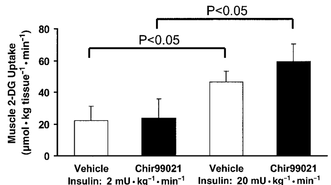
FIG. 6. In vivo rates of 2,6- 3 H-2-deoxy-D-glucose uptake in gastrocnemius muscle in ZDF ( fa/fa ) rats treated with vehicle (□) or CHIR99021 (■) after euglycemic-hyperglycemic clamps at insulin infusion rates of 2 or 20 mU · kg -1 · min -1 .
