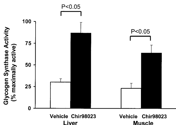
FIG. 3. Percent of maximally active form of glycogen synthase in liver and muscle of ZDF ( alfa ) rats treated with vehicle (□) or CHIR98023 (■) after an OGTT. * P < 0.05.
