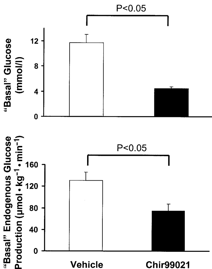
FIG. 7. Fasting blood glucose concentration (A) and rates of EGP (B) in diabetic ZDF ( fa/fa ) rats after a 20-h infusion of either vehicle (□) or CHIR99021 (■).
