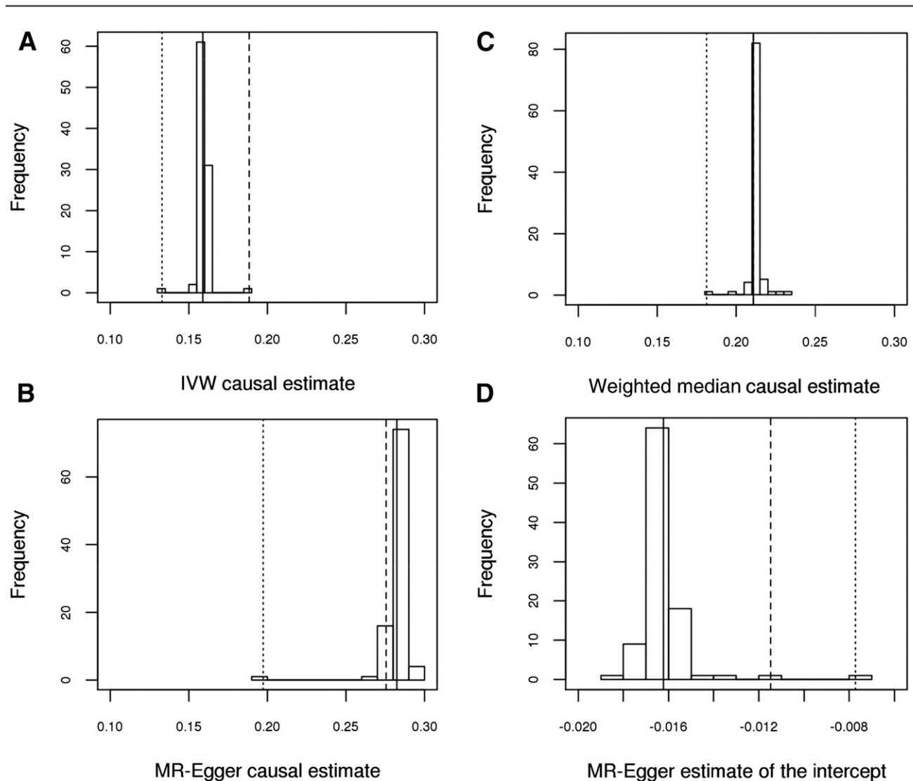
Figure 2 —Distributions of regression estimates resulting from leave-one-out permutation analysis. Solid line, estimate from main analysis ( n = 96 variants); dashed line, estimate with TCF7L2 (rs7903146) removed; dotted line, estimate with FTO (rs1558902) removed. A: Causal estimates ( \beta -coefficients) of BMI on type 2 diabetes estimated by an IVW method. B: Causal estimates ( \beta -coefficients) of BMI on type 2 diabetes estimated by MR-Egger. C: Causal estimates ( \beta -coefficients) of BMI on type 2 diabetes estimated by a weighted median method. D: Estimates of the intercept by MR-Egger.
