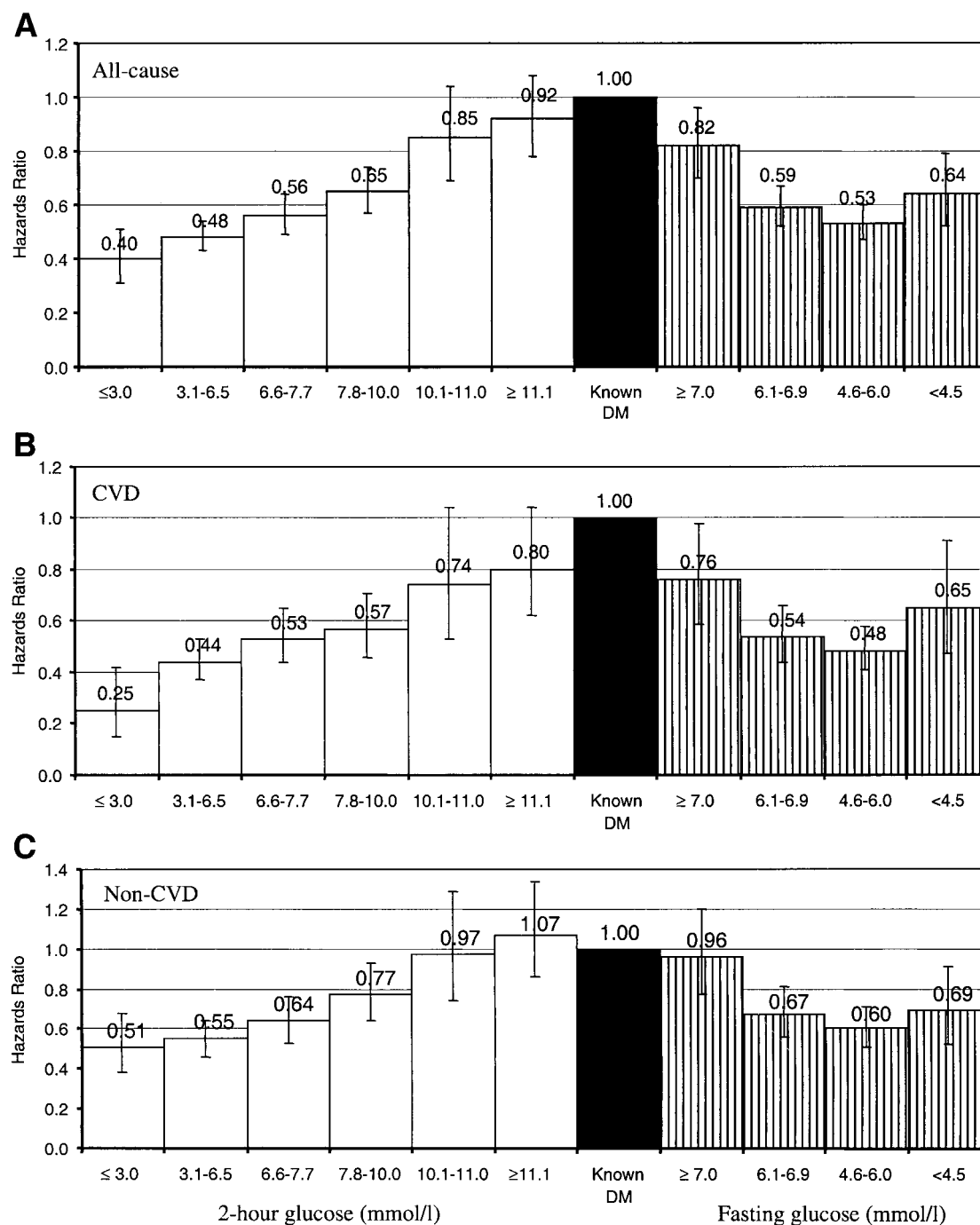
Figure 3 —HRs (columns) and 95% CIs (vertical bars) for mortality from all causes (A), CVD (B), and non-CVD (C) for the FPG and 2hPG intervals using previously diagnosed diabetes as a common reference category, adjusted for age, sex, cohorts, BMI, systolic blood pressure, cholesterol, and smoking.
