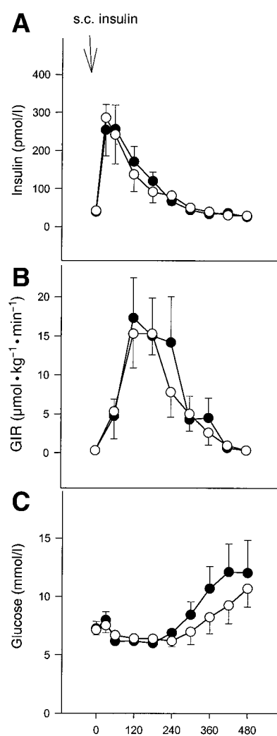
Figure 2 —A: Serum insulin levels before and after subcutaneous injection (at 0 min) of insulin aspart (●) or insulin lispro (○) in seven patients with type 1 diabetes. Data are means ± SEM. B: GIR needed to prevent hypoglycemia in the same seven patients. C: Plasma glucose concentrations before and after subcutaneous injection of insulin aspart or insulin lispro in the same seven patients.
