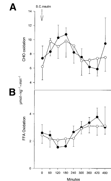
Figure 4 —Rates of carbohydrate (A) and FFA oxidation (B) before and after subcutaneous injection (at 0 min) of either insulin aspart (●) or insulin lispro (○) in seven patients with type 1 diabetes.
