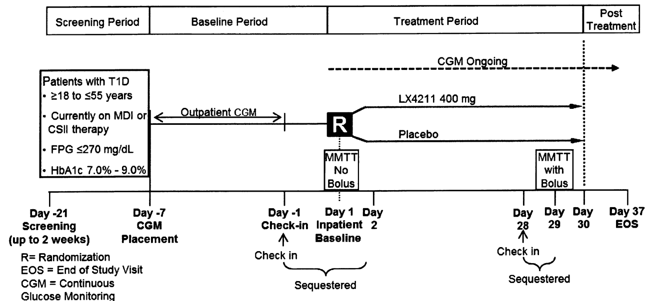
Figure 1—Study design.
