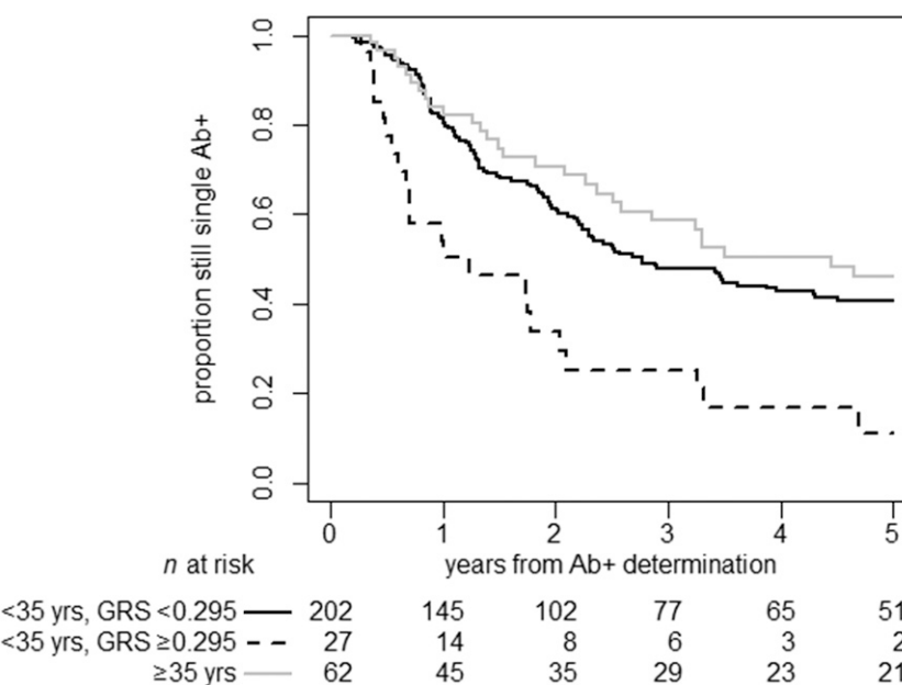
Figure 4 —Time from single to multiple islet autoantibody positivity (Ab+) in relatives of patients, by age ( < 35 vs. \geq 35 years) and T1D GRS group ( < 0.295 vs. \geq 0.295 ) ( P = 0.0001 ). While the T1D GRS did not further increase the predictive ability in participants aged \geq 35 years, it was able to stratify risk in individuals aged < 35 years.
