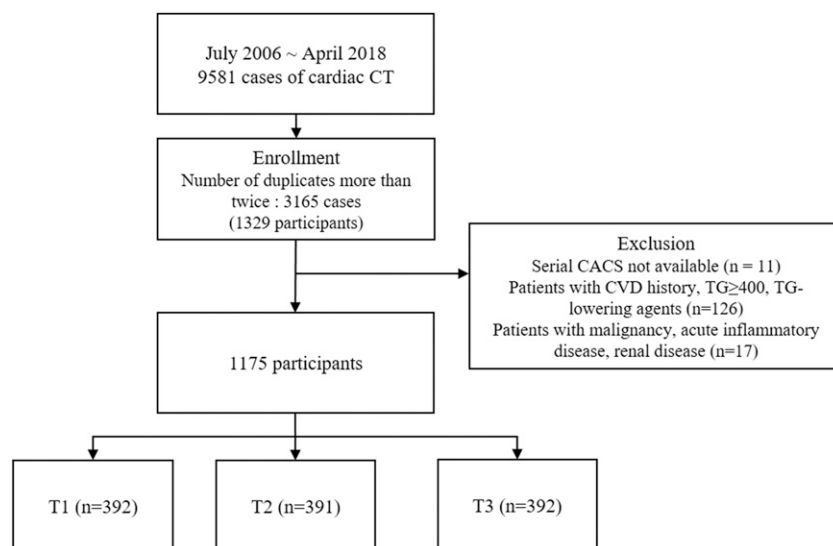
Figure 1—Study flow.
