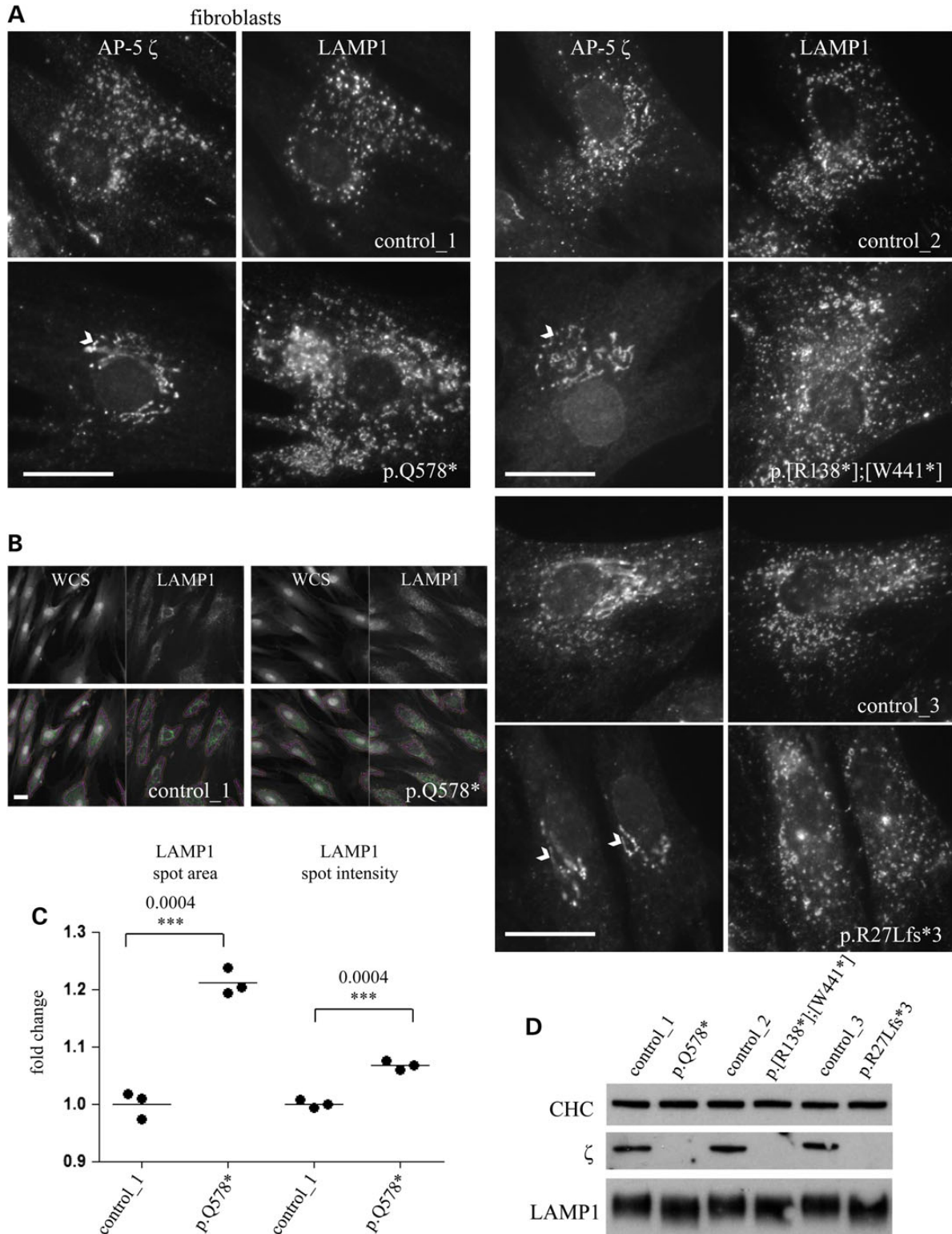
Figure 2. Loss of AP-5 in patient-derived fibroblasts. (A) Immunofluorescence of patient-derived fibroblasts (denoted by their mutation) and their respective gender- and age-matched controls double-labelled with antibodies against AP-5 \zeta and LAMP1. Note that in control cells there is a significant overlap between LAMP1 and AP-5 \zeta . In AP5Z1 patient lines, there is loss of the punctate AP-5 labelling pattern [the antibody cross-reacts with a reticular Golgi protein (white arrowhead), and this immunoreactivity persists when cells are depleted of AP-5 \zeta by siRNA knockdown (4)]. Note that with the loss of AP-5 \zeta , there is a consistent increase in the brightness and size of the LAMP1-positive puncta. Scale bar = 20 \mu m. (B) Patient-derived fibroblasts (p.Q578*) and their control (control_1) were plated onto 96-well plates and labelled with a whole-cell stain (WCS) and an antibody against LAMP1; the WCS allowed a mask to be drawn around the cells (pink) and various parameters of LAMP1 puncta (green) to be quantified on an ArrayScan Cellomics microscope using a SpotDetector algorithm. Scale bar = 20 \mu m. (C) Spot average intensity and average area per object were quantified in three independent experiments, with more than 1000 cells quantified per experiment. Note that there is a subtle but significant increase in the area of the LAMP1-positive puncta. (D) Western blots of patient-derived fibroblasts probed for LAMP1, AP-5 \zeta and clathrin (CHC; loading control). Note that there is no apparent increase in the total levels of LAMP1 protein.
