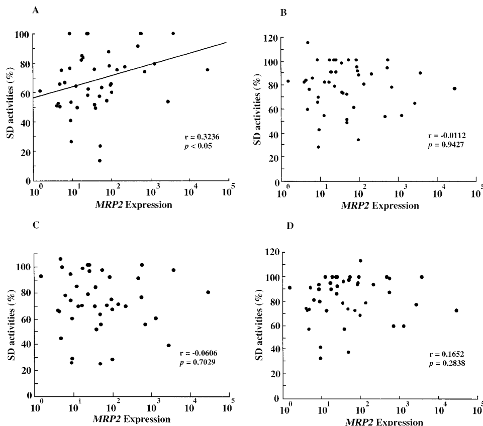
Fig. 3 Correlation between MRP2 mRNA expression and succinate dehydrogenase activity of cisplatin (A), 5-fluorouracil (B), mitomycin C (C), and doxorubicin (D). The Spearman's correlation coefficient ( r ) and associated probability ( P ) were calculated for each combination of MRP2 mRNA expression and succinate dehydrogenase activity. SD , succinate dehydrogenase.
