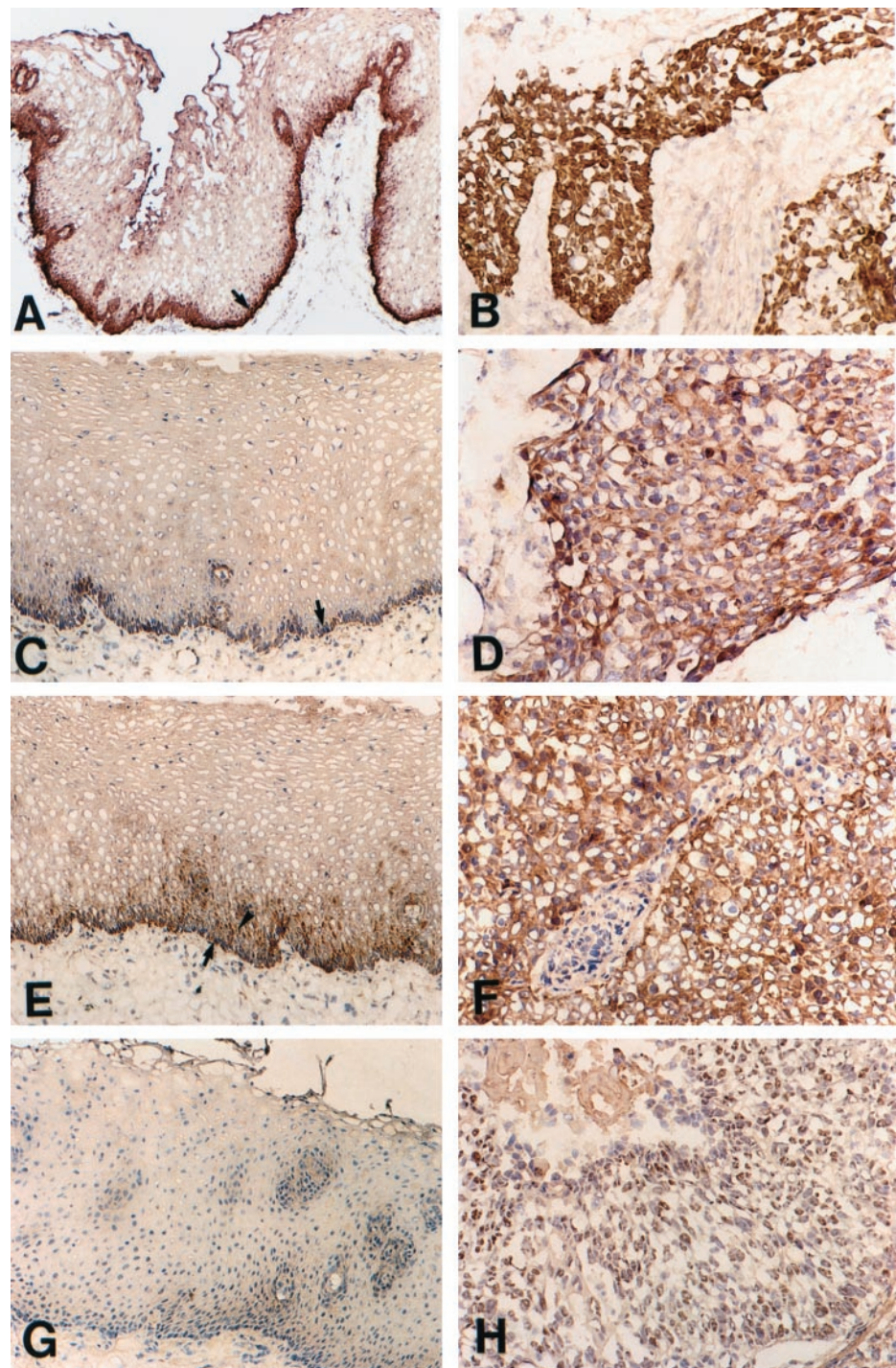
Fig. 3 Photomicrographs of Fra-1 , neogenin , Id-1 , and CDC25B expression by IH in morphologically normal esophageal epithelium and ESCC. A , Fra-1 IH in morphologically normal esophageal epithelium showing that Fra-1 expression was restricted to the basal cell layer (arrow); DAB \times 160 . B , Fra-1 IH in ESCC showing that the nuclei of tumor cells are strongly positive for Fra-1 ; DAB \times 400 . C , Neogenin IH in morphologically normal esophageal epithelium showing that Neogenin expression was restricted to the basal cell layer (arrow); DAB \times 330 . D , Neogenin IH in ESCC showing Neogenin expression in the cytoplasm of tumor cells; DAB \times 500 . E , Id-1 IH in morphologically normal esophageal epithelium showing Id-1 expression was restricted to the basal (arrow) and parabasal (arrowhead) cell layers; DAB \times 330 . F , Id-1 IH in ESCC showing Id-1 expression in the cytoplasm of tumor cells; DAB \times 500 . G , CDC25B IH in morphologically normal esophageal epithelium showing lack of immunoreactivity; DAB \times 330 . H , CDC25B IH in ESCC showing CDC25B expression in the nuclei of most tumor cells; DAB \times 500 .
