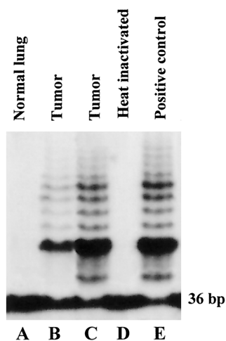
Fig. 1 Telomerase activity in NSCLC, normal lung tissue, and control samples. The 36-bp internal positive control band is seen in every lane. Lane A, telomerase-negative normal lung tissue extract showing only the 36-bp band. Lanes B and C, representative telomerase-positive NSCLC extracts showing the ladder pattern of PCR products, similar to that seen in Lane E (telomerase-positive control cell extract). Lane D, heat-inactivated telomerase-positive NSCLC extract.
