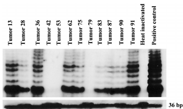
Fig. 2 Telomeric repeat amplification protocol analyses of NSCLC specimens are shown (Tumors 13–91). Tumors 42, 53, and 79 are examples of telomerase-negative lung carcinomas; the other tumor samples represent telomerase-positive cases. The last two lanes correspond to a heat-inactivated telomerase-positive NSCLC extract and to the telomerase-positive control cell extract.
