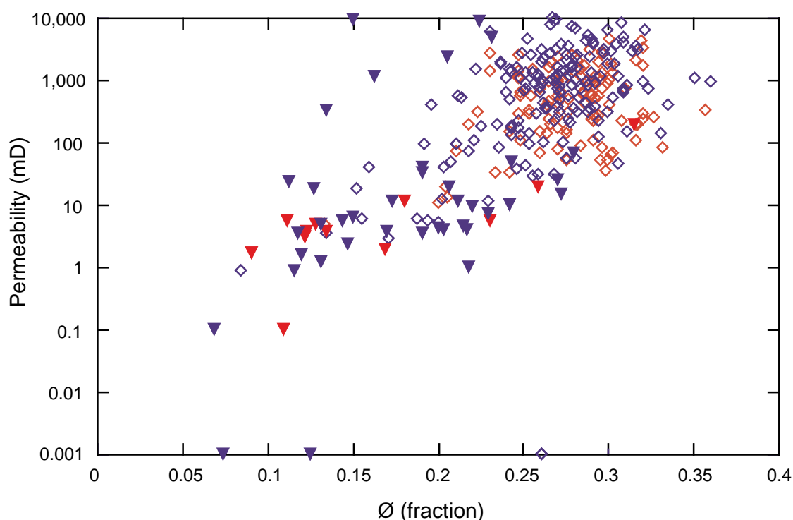
Figure 4: Relationship between porosity and permeability for specific rock-fabric units from two North 'Ain Dar cores. Note that grainstones and mud-lean packstones (open diamonds) plot in a distinct porosity-permeability field relative to packstones, wackestones, and mudstones (solid triangles). Core plug data from upper third of reservoir; dolomite plugs have been excluded.
