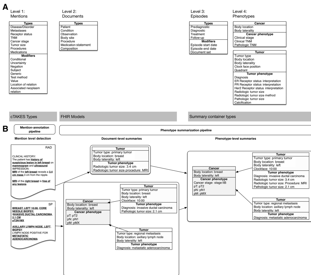
Figure 1. Domain model (A) and example of phenotypes produced from the DeepPhe system (B). Bold and underlined items in B show the mentions extracted by cTAKES pipeline 1 (mention detection). cTAKES, Apache Clinical Text Analysis and Knowledge Extraction System; FHIR, Fast Healthcare Interoperability Resources; RAD, radiology note; SP, surgical pathology note.
