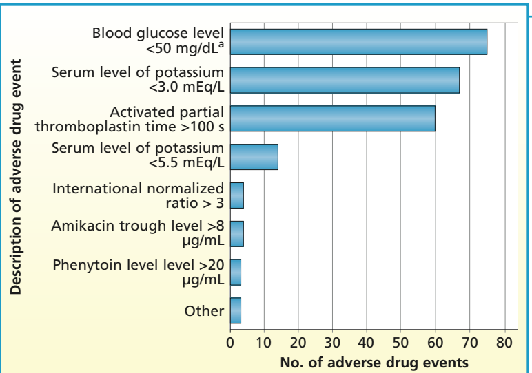
Figure 1 Characteristics and numbers of adverse drug events ( N = 230 ). The category Other includes 1 case of vancomycin peak level exceeding 40 \mu g/mL, 1 case of tacrolimus level exceeding 20 ng/mL, 1 case of cyclosporine trough level exceeding 300 \mu g/mL, and no cases of a valproate level exceeding 100 \mu g/mL.
