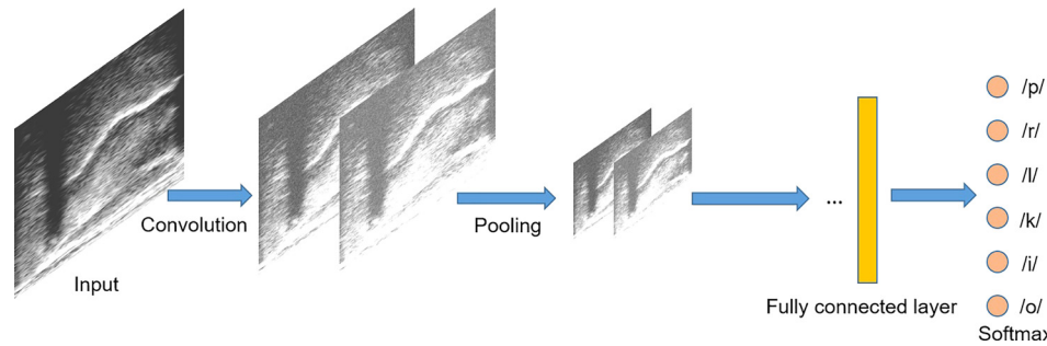
Fig. 2. (Color online) An example architecture of a Convolutional Neural Network for the classification task. The ellipsis denotes the subsequent convolutional and pooling layers.
