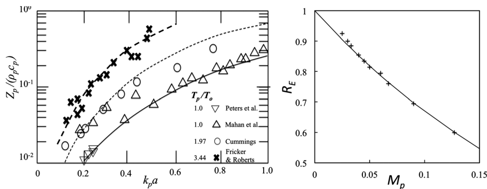
Fig. 1. (a) Influence of temperature on the open pipe termination Z_p as a function of the Helmholtz number k_p a in the limit M_p \rightarrow 0 [Eq. (10)]. Theory T_p/T_o = 1.0 (line —) compared to the data of Mahan et al. (Ref. 10) ( \Delta ) and Peters et al. (Ref. 6) ( \nabla ) at room temperature. Theory T_p/T_o = 1.97 (line ····) compared to the data of Cummings (Ref. 9) ( \circ ) at T_p = 573 K. Theory T_p/T_o = 3.44 (line - - - -) compared to the data of Fricker and Roberts (Ref. 8) ( \times ) at T_p = 1273 K. (b) Influence of the surface averaged Mach number M_p on the energy reflection coefficient at room temperature T_p = T_o . The experimental data at low Strouhal numbers 0.065 \leq k_p a/M_p \leq 0.33 ( + ) has been obtained by Hirschberg and Rienstra (Ref. 24) using the same setup as Peters et al. (Ref. 6). Theory (line —) was calculated using Eq. (9) with |R| = 1 and the cross sectional averaged Mach number M_p .
