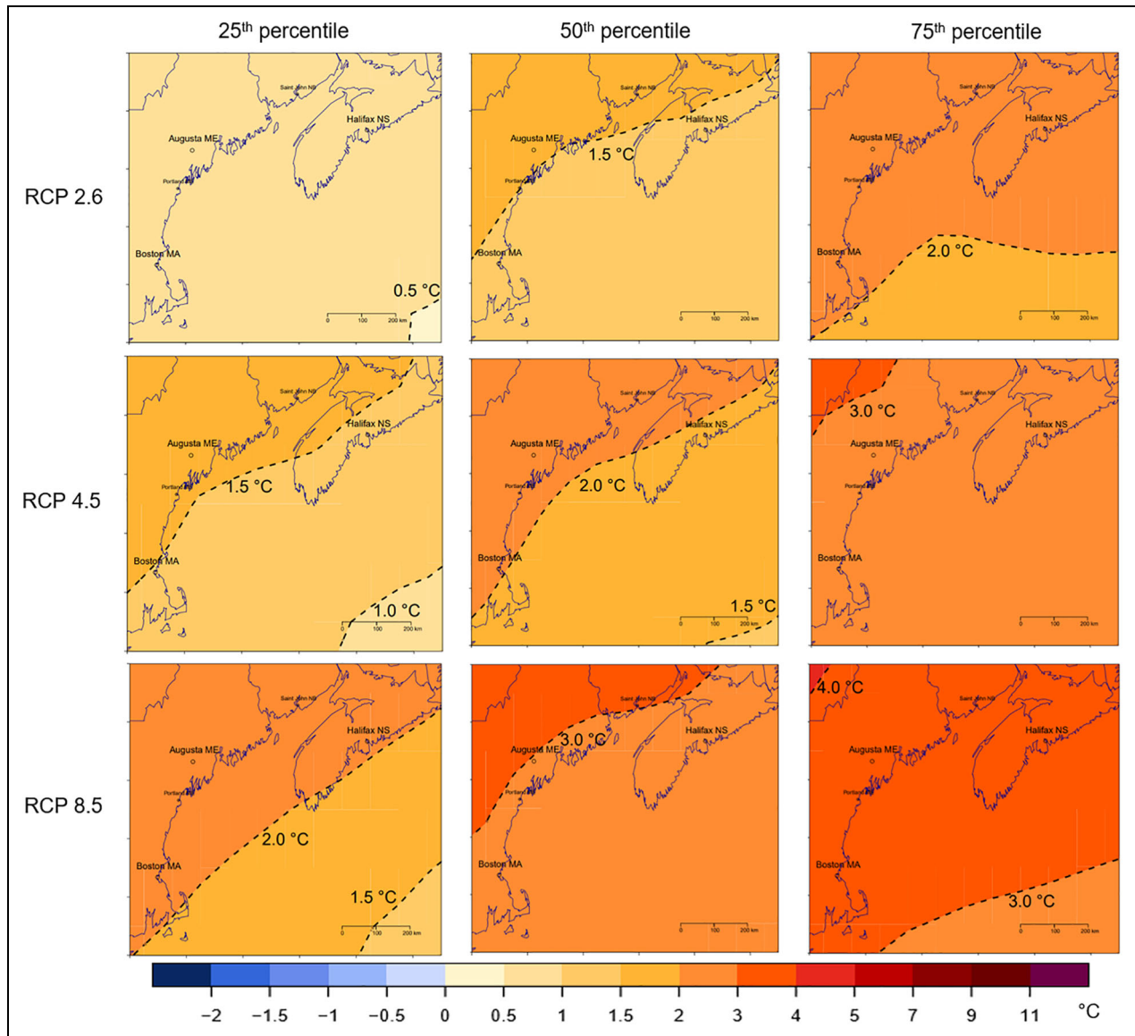
Figure 1. Spatial depiction of projected changes (relative to 1986–2005) in annual mean air temperature. Based on CMIP5 multi-model ensemble results for the GOM region ( 1 \times 1^\circ grid resolution) for 2046–2065 for three scenarios (RCP2.6, RCP4.5, and RCP8.5) and for three percentiles (25th, 50th, and 75th). DOI: https://doi.org/10.1525/elementa.2021.00059.f1
