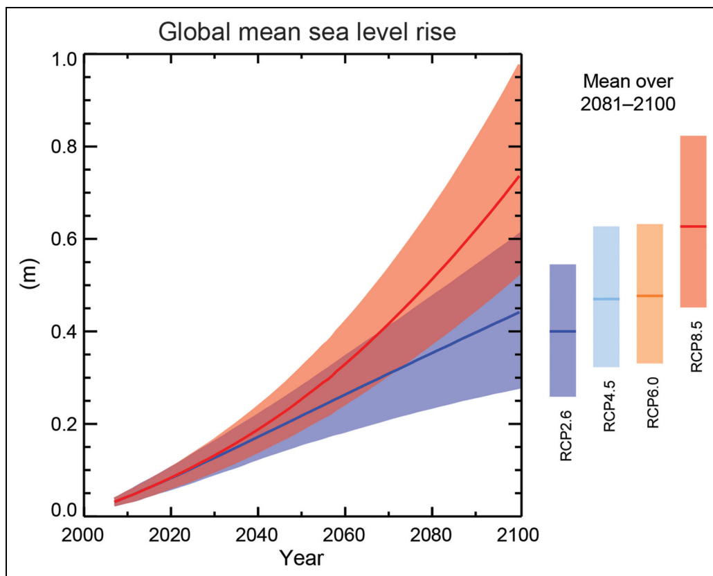
Figure 2. Projected change in global mean sea levels due to climate change. Projections of global mean sea-level rise over the 21st century relative to 1986–2005 from the combination of the CMIP5 ensemble with process-based models, for RCP2.6 and RCP8.5. The assessed likely range is shown as a shaded band. The assessed likely ranges for the mean over the period 2081–2100 for all RCP scenarios are given as colored vertical bars, with the corresponding median value given as a horizontal line (IPCC, 2013b, Figure SPM.9). DOI: https://doi.org/10.1525/elementa.2021.00059.f2
