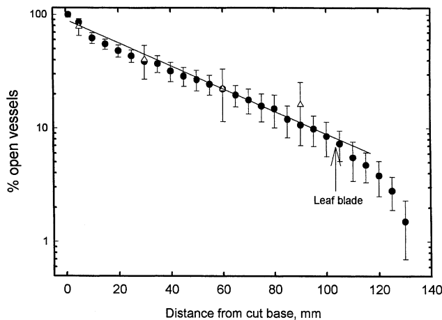
Fig. 1. Solid circles are a plot of open-vessel length distribution in sunflower petioles obtained by paint perfusion. The error bars are standard error values n=7 . Open triangles are from embolized vessel counts in the cryo-SEM at distances of 5, 30, 60, and 90 mm. The error bars at these distances are the standard error of the cryo-SEM counts.
