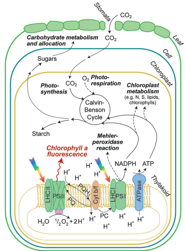
Fig. 7. Schematic representation showing the interactions of the main processes in \text{C}_3 photosynthesis in higher plants. Photophosphorylation starts with the absorption of light by the light-harvesting antenna complexes (LHCI and LHCII) associated with photosystem II (PSII) and photosystem I (PSI) in the chloroplast thylakoid membrane. This drives electron transport from water via a series of electron carriers to NADP, producing reducing power (NADPH) and a \text{H}^+ electrochemical potential difference across the membrane. Dissipation of this proton motive force by the passage of \text{H}^+ back across the membrane through the ATPase drives the production of ATP. Ribulose 1,5-bisphosphate carboxylase/oxygenase (Rubisco) catalyses the assimilation of \text{CO}_2 with ribulose 1,5-bisphosphate (RubP) in the carboxylation reaction of the Calvin-Benson cycle in the stroma of the chloroplast. The diffusion of atmospheric \text{CO}_2 into the leaf is regulated by the stomata in the epidermis. Other reactions of the Calvin-Benson cycle utilize NADPH and ATP to produce triose phosphates which are required for the synthesis of carbohydrates. NADPH and ATP are also used in a range of other metabolic activities (e.g. nitrogen and sulphur metabolism, lipid and pigment synthesis) in the chloroplast. Rubisco can also catalyse the photorespiratory oxygenation of RubP, which involves consumption of NADPH and ATP by the Calvin-Benson cycle. \text{O}_2 can also be directly photoreduced by electron transfer from PSI to produce superoxide which is then rapidly dismutated to hydrogen peroxide, which in turn is detoxified to water; this process is often termed the Mehler-peroxidase reaction or the water-water cycle. Cyt b/f , cytochrome b 6 f complex; PC, plastocyanin; PQ, plastoquinone; \text{PQH}_2 , plastoquinol.
