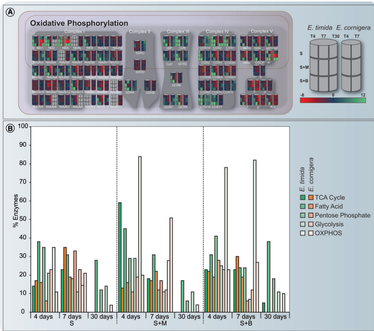
Fig. 2. —Gene expression changes in the OXPPOS and other mitochondrion-related pathways. (a) Gene expression shifts of the OXPPOS metabolic pathway. KEGG-based map of oxidative phosphorylation. Coloured “barrels” displays gene expression levels for starving E. cornigera and E. timida starved for 4, 7, and 30 days (T4, T7, T30) relative to the freshly fed state; upregulation is shown from green to blue, downregulation from blue to red, and grey boxes indicate no detectable gene expression for the given condition. Each barrel represents an enzyme, with the wider barrels representing E. timida due the extra data point of day 30 (T30). Multiple barrels at one step in the metabolic pathway represent a protein complex (e.g., complex I); note that one enzyme (or complex) can act at multiple steps in the pathway and in different complex compositions. For every enzyme (complex) the two species are shown adjacent to each other for comparison. Relevant substrates are indicated by dots and labelled with their common name. Note some steps of the fatty acid pathway occur in the mitochondrion. (b) Frequency of upregulation among metabolic pathway-associated gene expression. Bardigram of the percentage of upregulation (relative to T_0 : \log_2[FC_{condition/T_0}] \geq 1 ) of gene expression associated with the 5 main mitochondrial energy metabolism pathways; all enzymes of one pathway are added up to represent 100%. Note that only in the case of oxidative phosphorylation (OXPPOS) in E. timida (and with either monolinuron or bleaching treatment), 80–100% of the associated enzymes are observed to be upregulated. This might reflect a response of the animal to an increase of reactive oxygen species actually stemming mainly from abiotically stressed kleptoplasts and not the mitochondria themselves. For details please refer to the text. TCA, tricarboxy acid cycle; S, starvation alone; S + M, starvation with additional 2 µg/ml of the photosynthesis inhibitor drug monolinuron; S + B, starvation with a 1-h daily high light (1,000 µmol m -2 s -1 ) treatment.
