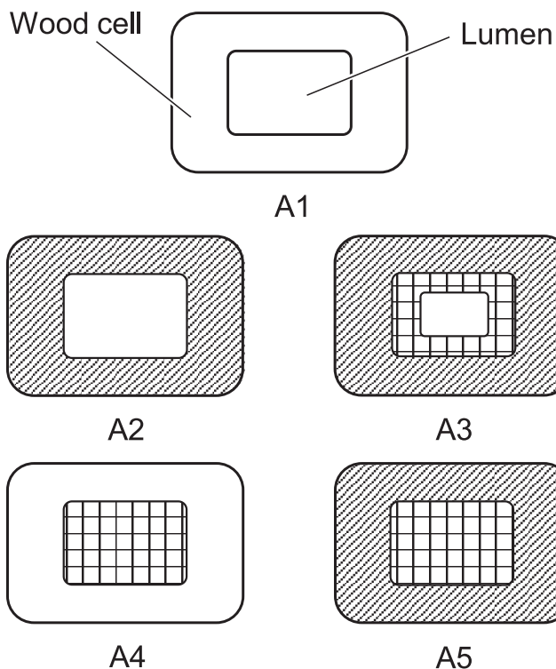
Figure 3.—Norimoto cell wall modification models (Norimoto 2001).
